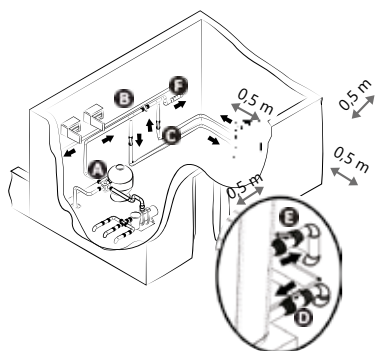
Innenmontage*
