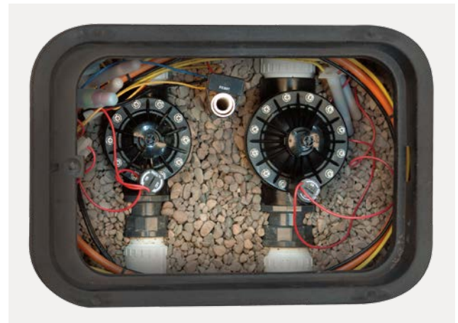
PGV Installed
